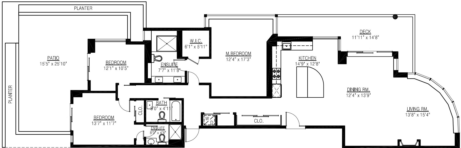
MAIN FLOOR PLAN FLOOR AREA: 1,851 sq.ft.
